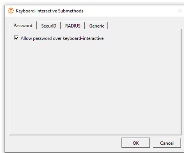
Figure 4.32. Keyboard-interactive submethods
