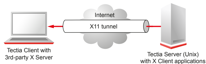
Figure 8.6. X11 forwarding
