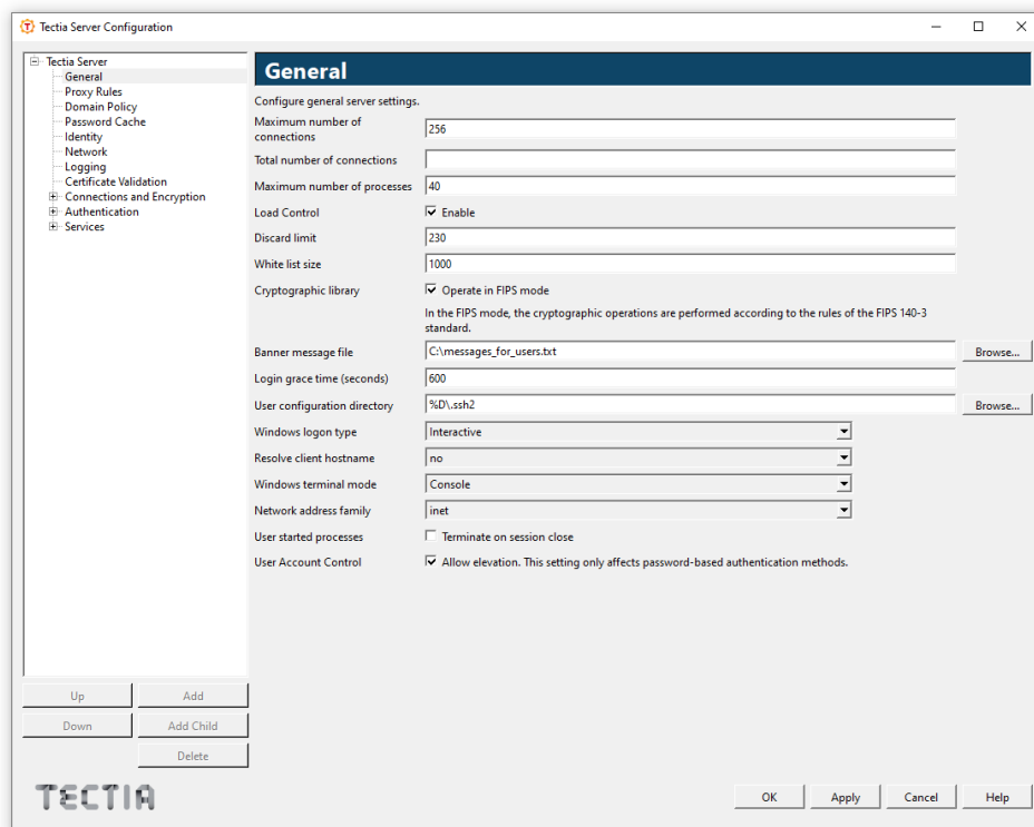
Figure 3.1. Activating FIPS mode on Tectia Server
