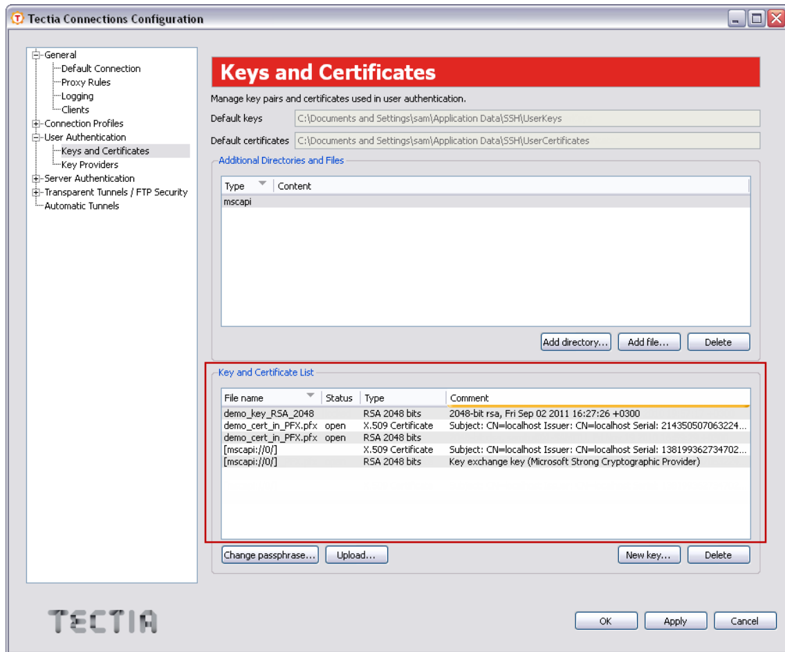
Figure 4.9. Viewing available certificates
