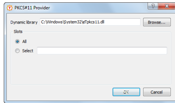
Figure A.29. Defining a PKCS #11 provider, Aladdin eToken DLL path shown as an example
