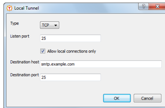
Figure A.25. Defining a local tunnel
