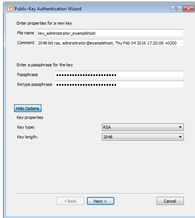
Figure A.16. The Public-Key Authentication Wizard
