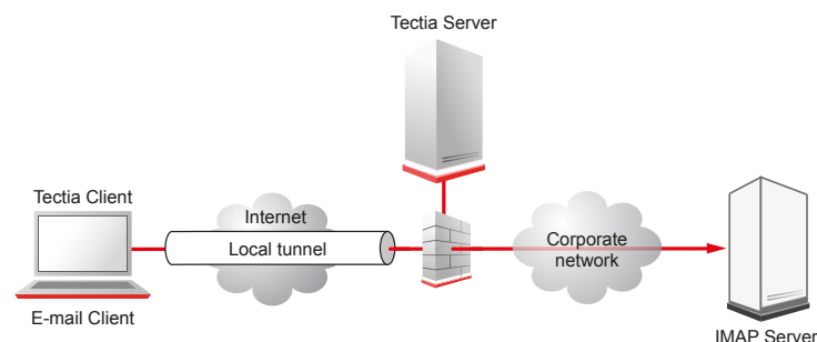
Figure 6.3. Local tunnel to an IMAP server
